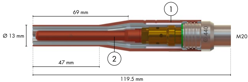
Narrow gap gas nozzle for ABIMIG® W / W T 440
