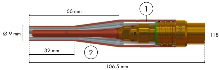
Narrow gap gas nozzle for ABIMIG® W / W T 340
